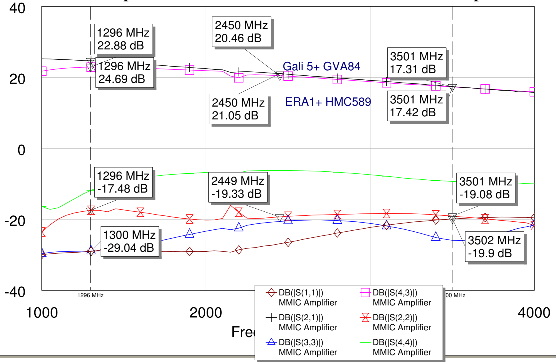
Graph of Gain & Return Loss for Dual MMIC Amp
