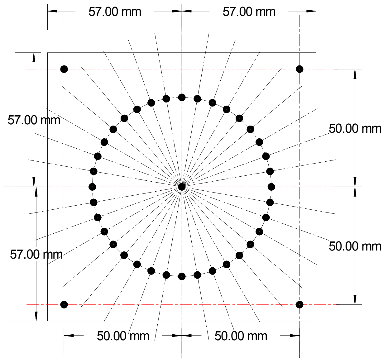
Drilling Template for 10deg placement LEDs on 38mm Rad ( 1.5" )
