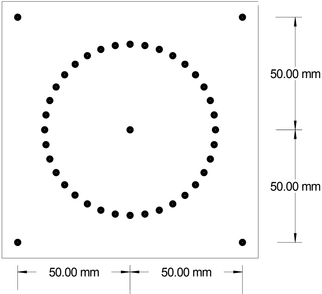
Drilling Template for 10deg placement LEDs on 38mm Rad ( 1.5" )
