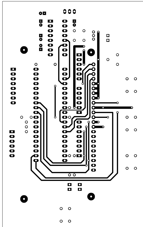
Top Copper
